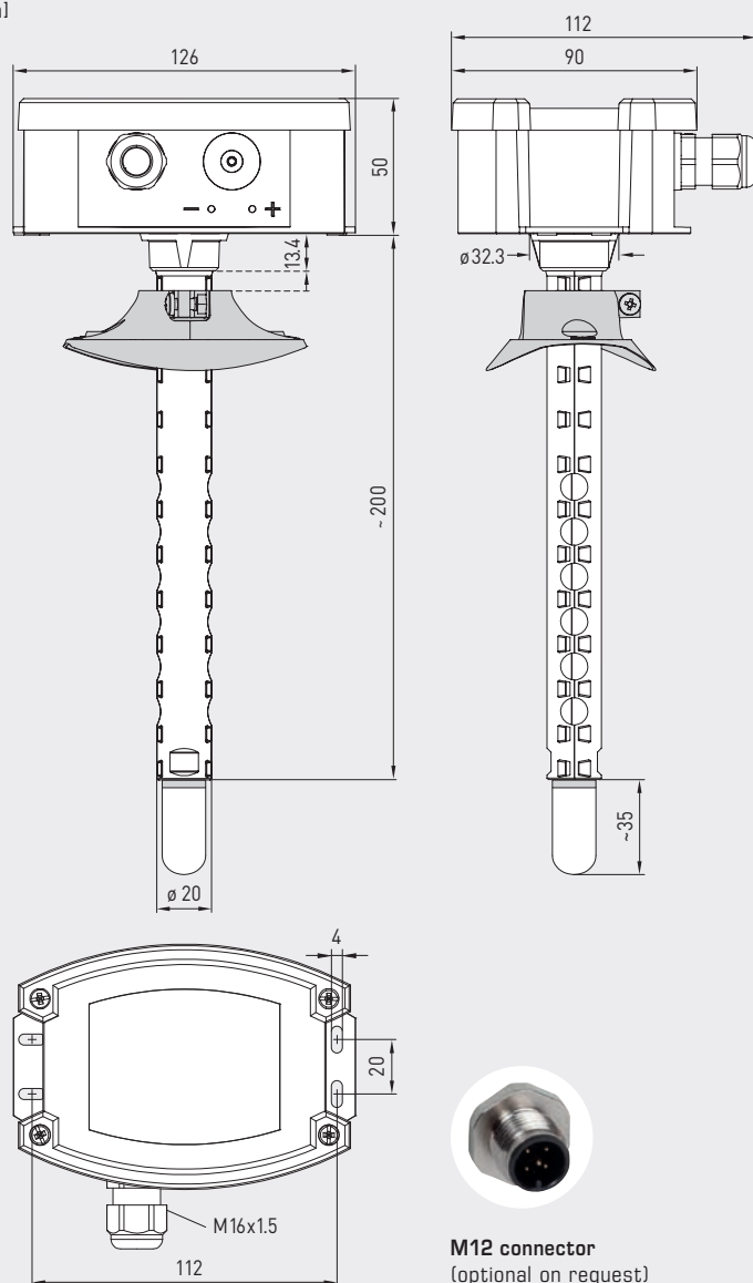
Dimensional drawing [mm]
