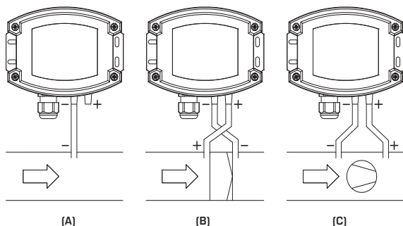
Mounting diagram
